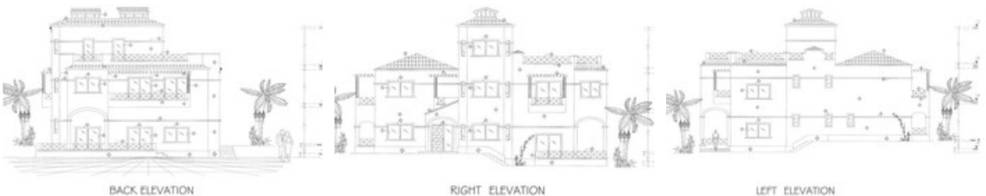
BACK ELEVATION
